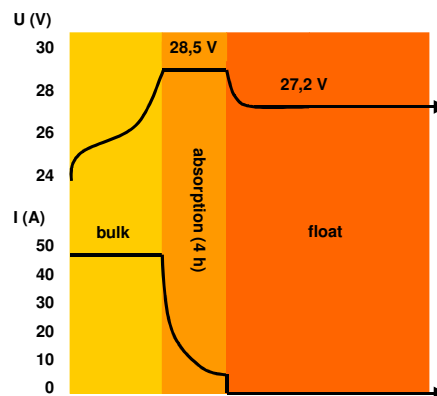
Charge curve
